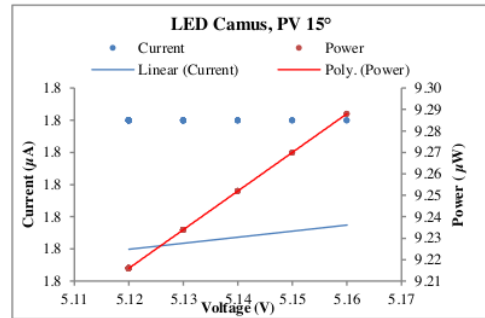
Figure 8. Power of monocrystalline PV panel at angle of 15° with 20 Watt Camus LED bulb radiation bulb radiations
